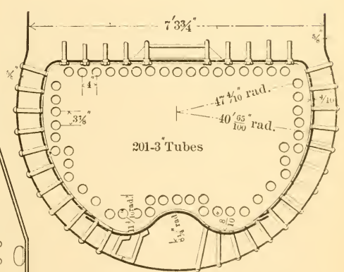
SECTION C-C LOOKING BACK
